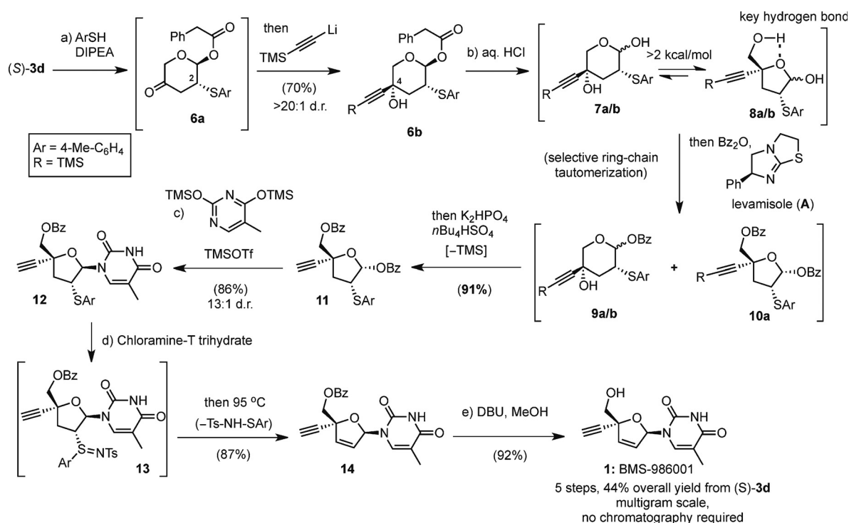
Scheme 2. Synthesis of BMS-986001 ( 1 ) from (S)- 3d . Reagents and conditions: a) p -thiocresol (1.1 equiv), i Pr 2 EtN (0.05 equiv), toluene, 20 °C, 30 min, then lithio-TMS-acetylene (2.5 equiv), THF (3.0 equiv), −78 °C, 1 h, 70%; b) 1 N HCl (0.5 equiv), CH 3 CN/H 2 O (5:1), 20 °C, 10 h, then Bz 2 O (3.0 equiv), levamisole (0.1 equiv), toluene, 20 °C, 48 h, then K 2 HPO 4 (3.0 equiv), nBu 4 HSO 4 (0.2 equiv), H 2 O (3.0 equiv), toluene, 0 °C, 1.5 h, 91%; c) bis(TMS)thymine (1.4 equiv), TMSOTf (1.4 equiv), CH 3 CN, 10 to 20 °C, 4.5 h, 86%, (13:1 d.r.); d) Chloramine-T (1.2 equiv), AcOH (0.1 equiv), CH 3 CN, 20 °C, 2.5 h, then nBuOH, 95 °C, 3 h, 87%; e) DBU (0.05 equiv), MeOH, 60 °C, 15 h, 92%. DBU = 1,8-diazabicyclo[5.4.0]undec-7-ene, Tf = trifluoromethanesulfonyl, THF = tetrahydrofuran, TMS = trimethylsilyl, Ts = 4-toluenesulfonyl.
